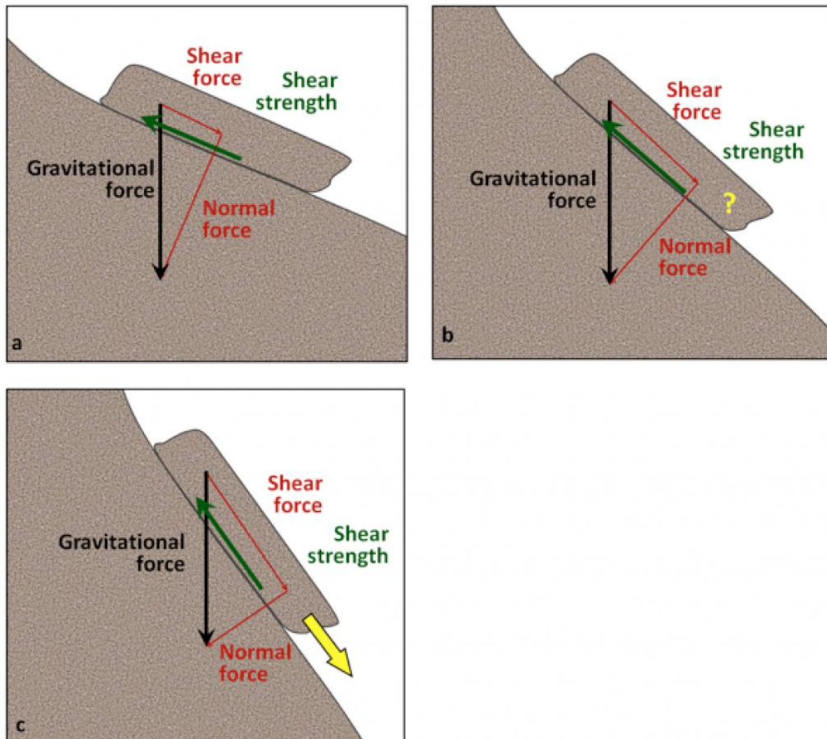
Figure 7.1.1 Differences in the shear and normal components of the gravitational force on slopes with differing steepness. The gravitational force is the same in all three cases. In (a) the shear force is substantially less than the shear strength, so the block should be stable. In (b) the shear force and shear
