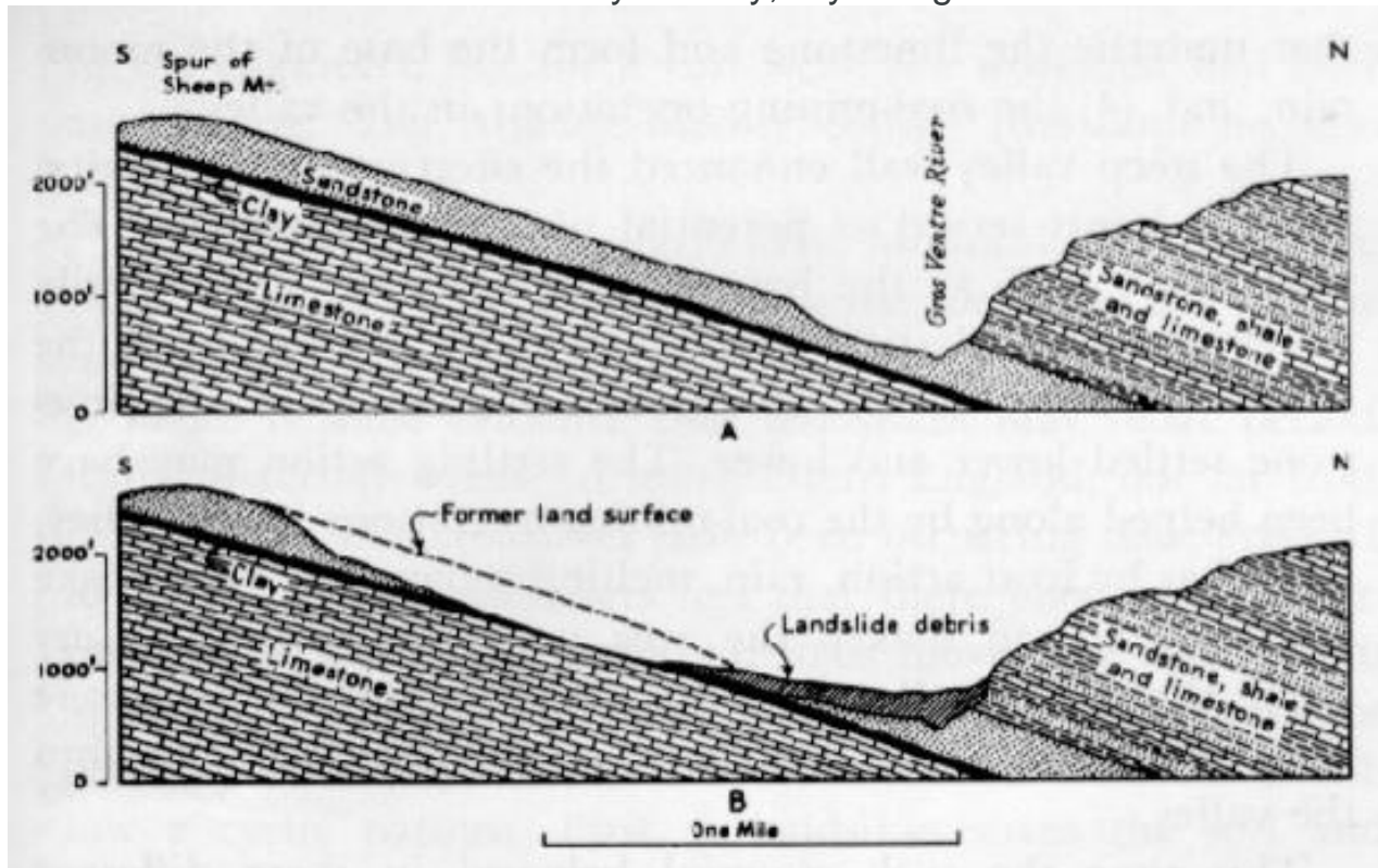
Figure 7.2.3 Cross-section of 1925 Gros Ventre slide showing sedimentary layers parallel with the surface and undercutting (oversteepening) of the slope by the river.
