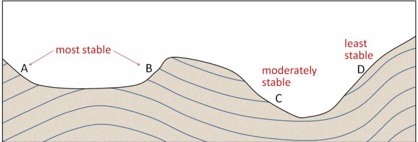
Figure 7.1.2 Relative stability of slopes as a function of the orientation of weaknesses (in this case bedding planes) relative to the slope orientations.
