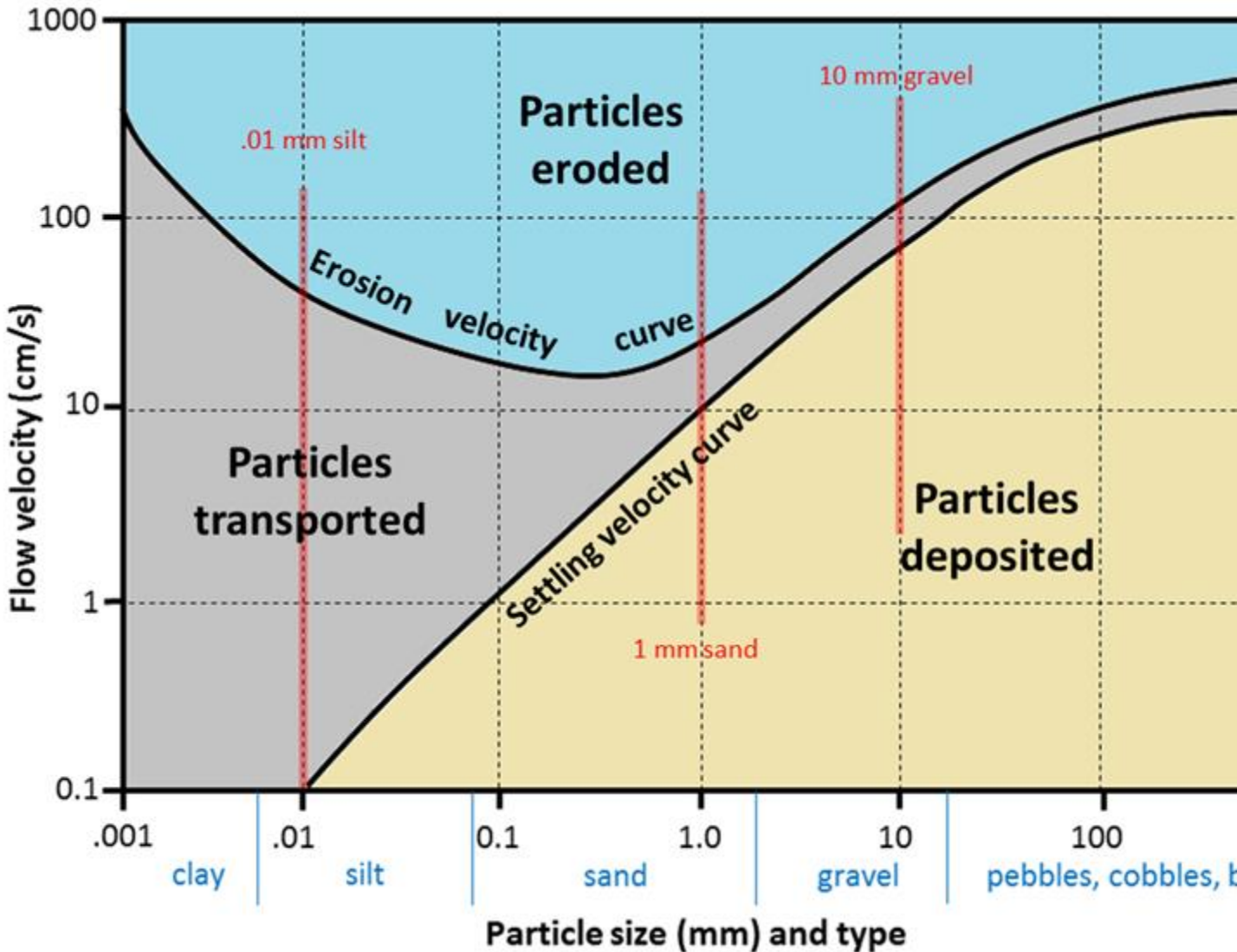
The Hjulström-Sundborg diagram showing the relationships between particle size and the tendency to be eroded, transported, or deposited at different current velocities. Steven Earle. CC-BY 4.0 International
