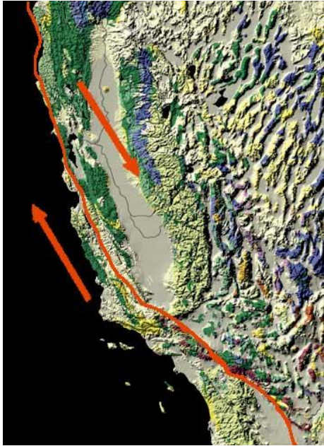
Figure 5.2.3 San Andreas Fault with plate motions. USGS, Public
