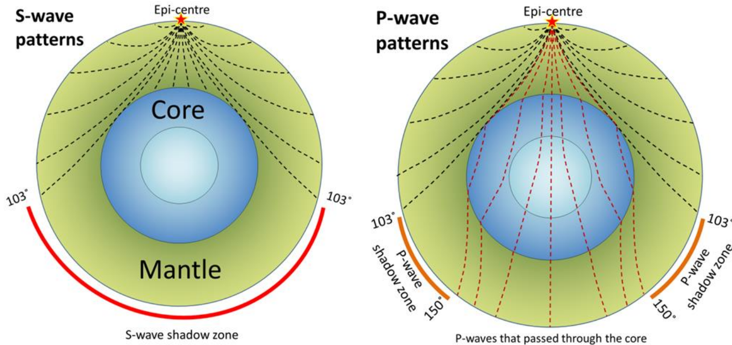
Figure 5.3.3 Patterns of seismic wave propagation through Earth's mantle and core. S-waves do not travel through the liquid outer core, so they leave a shadow on Earth's far side. P-waves do travel through the core, but because the waves that enter the core are refracted, there are also P-wave shadow zones. S Earle (2016) CC BY 4.0
