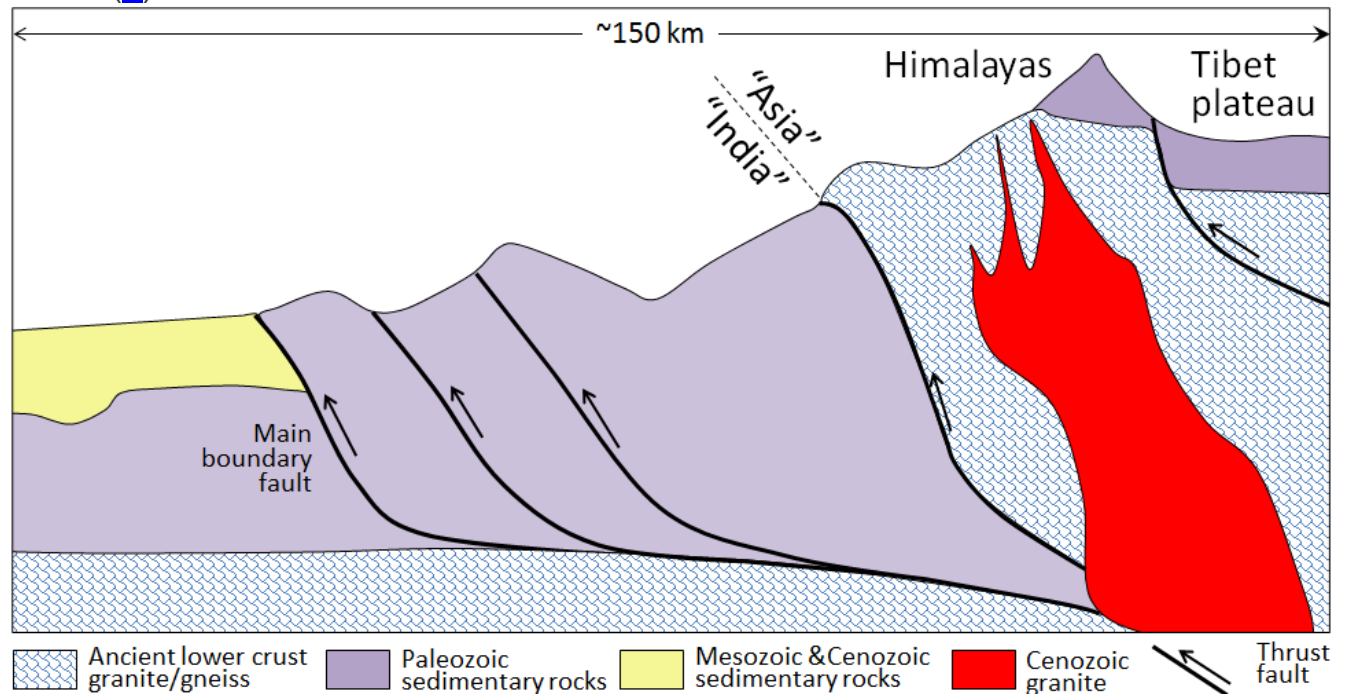
Figure 5.2.7 Schematic diagram of the India-Asia convergent boundary, showing examples of the types of faults along which earthquakes are focused. The devastating Nepal earthquake of May 2015 took place along one of these faults. Earle, CC-BY
