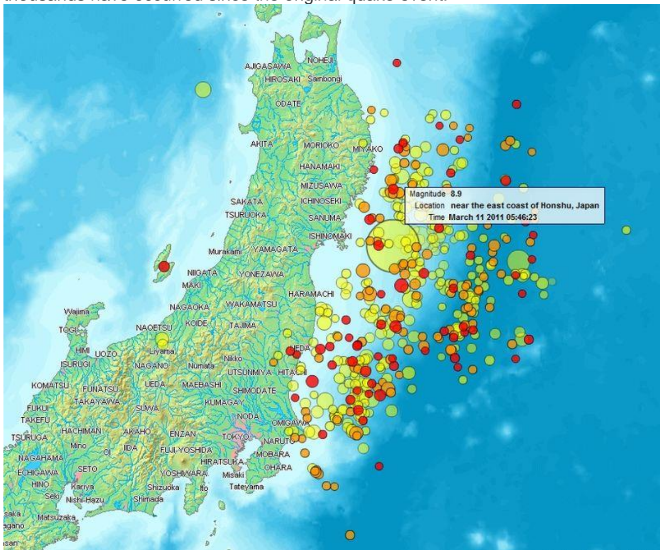
Figure 5.1.4. Map of the Sendai Earthquake, March 11, 2011 and aftershocks until March 14, 2011 at 11:20. The size of the circles is a function of magnitude, and the color indicates the date: light green: March 11; yellow: March 12; orange: March 13; red: March 14. Wikimedia Commons, Public Domain
