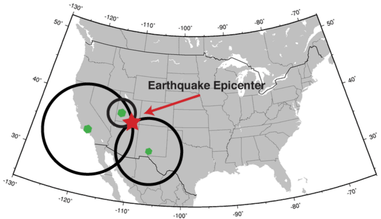
Figure 5.3.7 Triangulation can be used to locate an earthquake. The seismometers are shown as green dots. The calculated distance from each seismometer to the earthquake is shown as a circle. The location where all the circles intersect is the location of the earthquake epicenter. USGS, Public Domain
