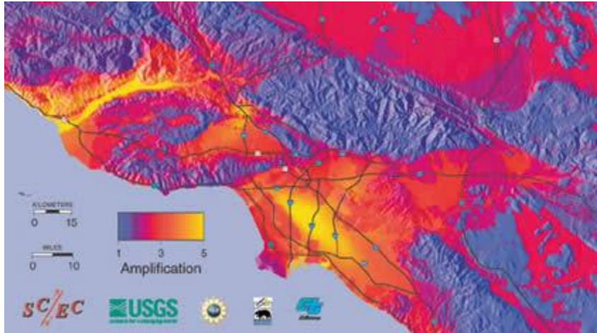
5.4.1 Map of Amplification in Los Angeles. USGS, Public Domain
