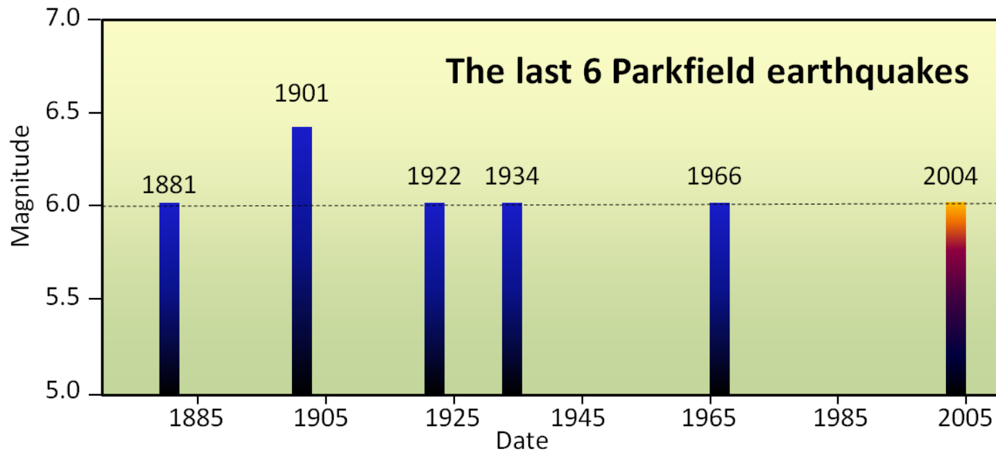
Figure 5.5.1 Earthquakes on the Parkfield segment of the San Andreas Fault between 1881 and 2004. S. Earle, CC-BY The U.S. Geological Survey recognized this as an excellent opportunity to understand earthquakes and earthquake prediction, so they armed the Parkfield area with a huge array of geophysical instruments and waited for the next quake, which was expected to happen around 1987. Nothing happened! The “1987 Parkfield earthquake” finally struck in September 2004 (Fig. 5.5.1). Fortunately all of the equipment was still there, but it was no help from the perspective of earthquake prediction. There were no significant precursors to the 2004 Parkfield earthquake in any of the parameters measured, including seismicity, harmonic tremor, strain (rock deformation), magnetic field, the conductivity of the rock, or creep, and there was no foreshock. In other words, even though every available technique was used to monitor it, the 2004 earthquake came as a complete surprise, with no
