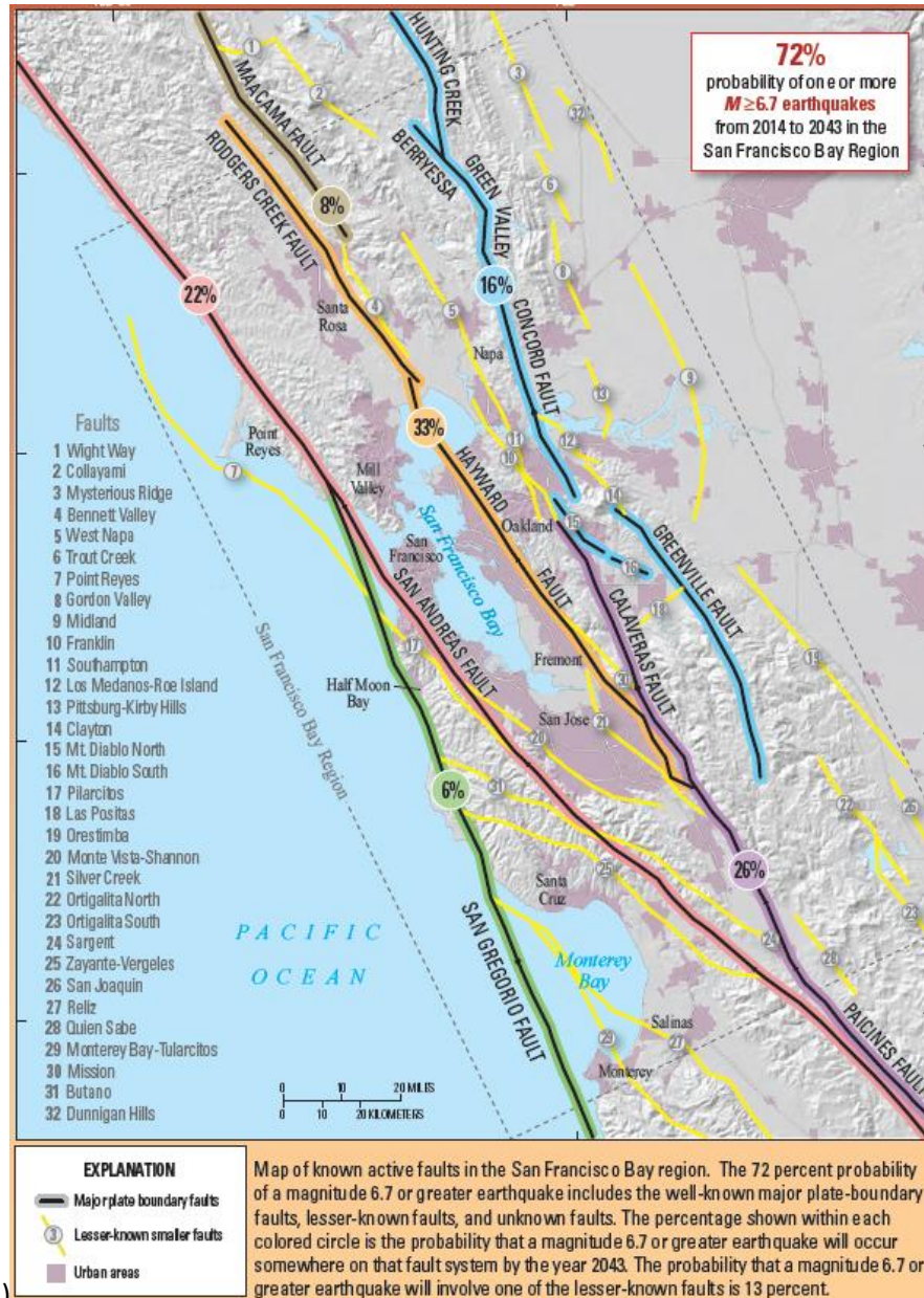
warning whatsoever. (5) Figure 5.5.2 Probabilities of a M6.7 or larger earthquake over the period 2014 to 2043 on various faults in the San Francisco Bay region of California. USGS, Public Domain
