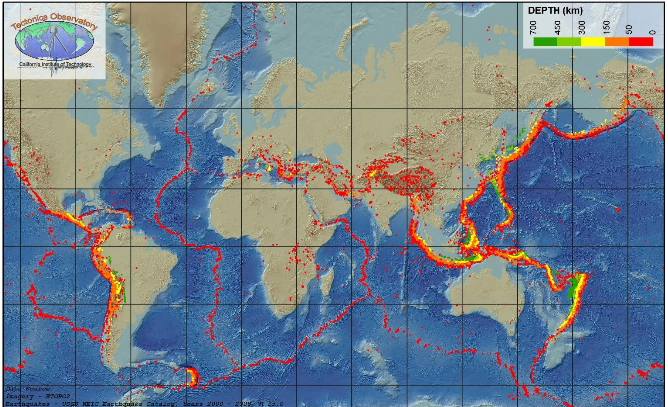
5.2.1 A global map of earthquake activity. The earthquakes occur at the boundaries between Earth's tectonic plates. The colors indicate the depth of the earthquakes, with red being the shallowest and green the deepest. Lisa Christiansen, Caltech Tectonics Observatory. CC-BY-NC
