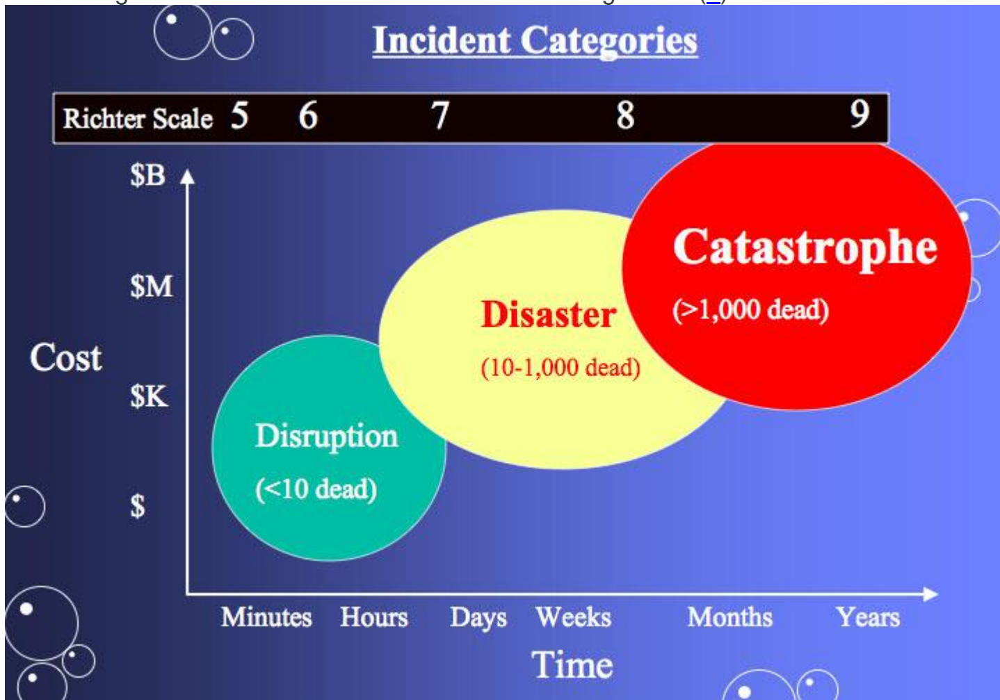
Earthquake Severity. Wikimedia Commons (2007), Public Domain.
