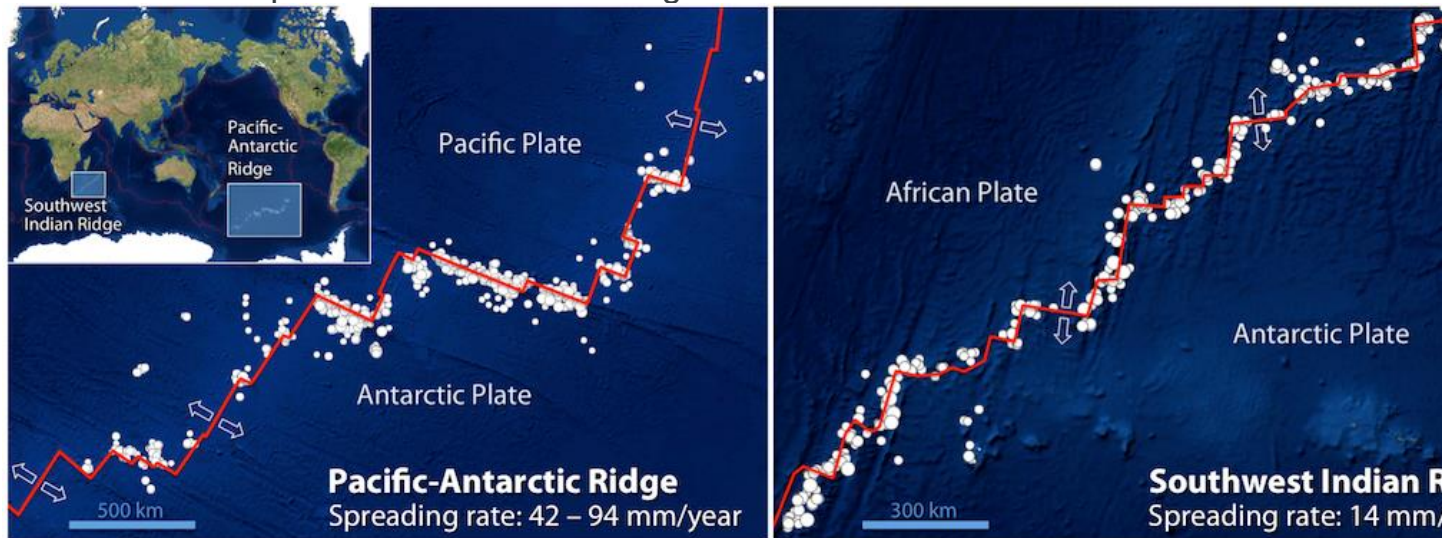
Figure 5.2.2. Locations of earthquakes of magnitude 4 and greater from 1990 to 2010 along two mid-ocean ridges. Plate boundaries are marked in red. Arrows show the direction of plate motion. Left: Rapidly spreading Pacific-Antarctic ridge with earthquakes concentrated along transform faults. Right: Slowly spreading Southwest Indian Ridge, with earthquakes along both spreading segments and transform faults. Karla Panchuk (2017) CC BY 4.0.
