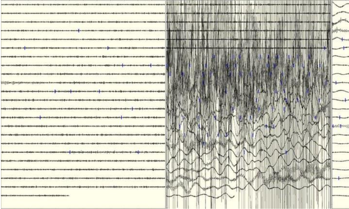
Figure 5.3.6 Multiple seismographs combined to show the dramatic movements from the magnitude 9.0 earthquake, Japan, 2011. Wikimedia Commons, CC-BY
