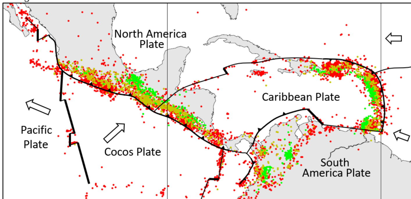
Figure 5.2.4 Distribution of earthquakes of M4 and greater in the Central America region from 1990 to 1996 (red: 0 to 33 kilometers depth, orange: 33 to 70 kilometers depth, green: 70 to 300 kilometers depth, blue: 300 to 700 kilometers depth) Spreading ridges are heavy lines, subduction zones are toothed lines, and transform faults are light lines. (Earthquakes Around the Mid-Atlantic Ridge © Steven Earle after Dale Sawyer, Rice University, CC-BY)
