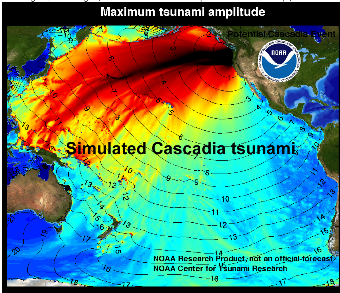
Figure 5.4.9 Maximum Tsunami Amplitude. A model of the tsunami wave heights (colors) and travel time contours from the 1700 Cascadia earthquake (M9). Tsunami wave amplitudes typically increase in shallow water. NOAA/PMEL/Center for Tsunami Research, Public domain.
