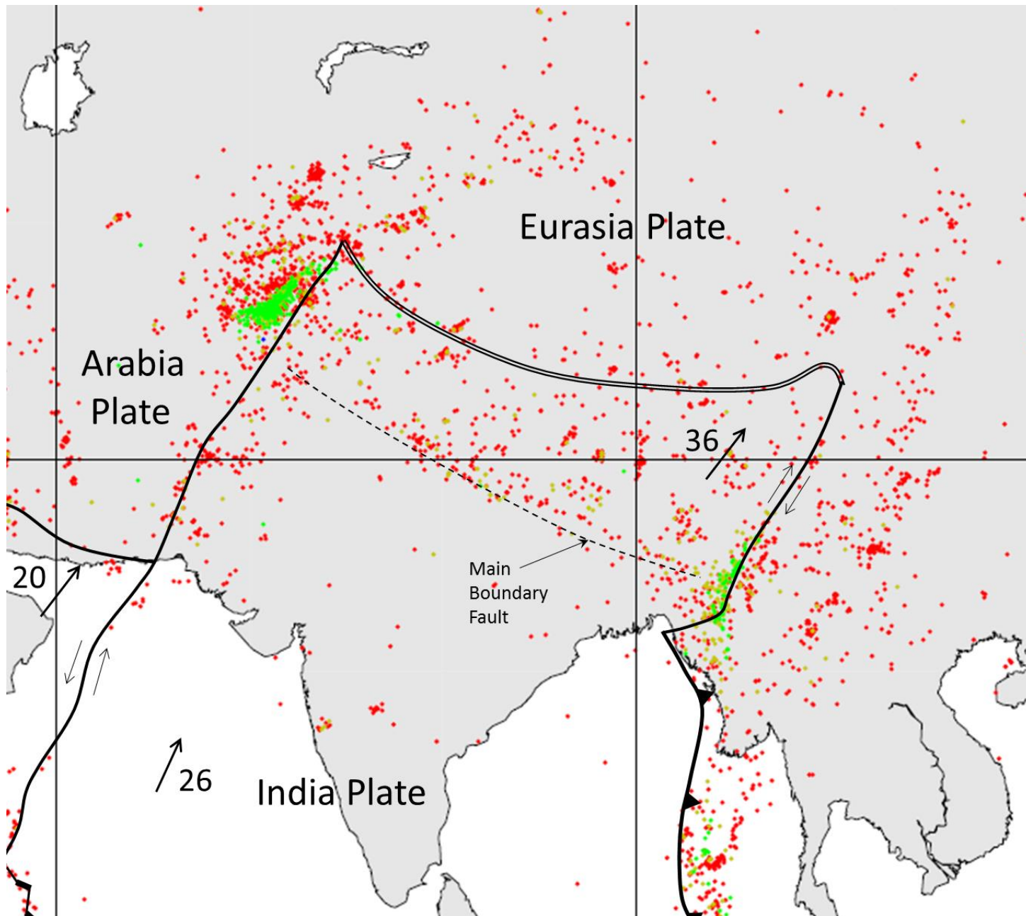
Figure 5.2.6. Distribution of earthquakes in the area where the India Plate is converging with the Asia Plate (data from 1990 to 1996, red: 0 to 33 kilometers, orange: 33 to 70 kilometers, green: 70 to 300 kilometers). The double line along the northern edge of the India Plate indicates convergence, but not subduction, and transform boundaries are seen on both sides. Plate motions are shown in millimeters per year. S. Earle, CC-BY
